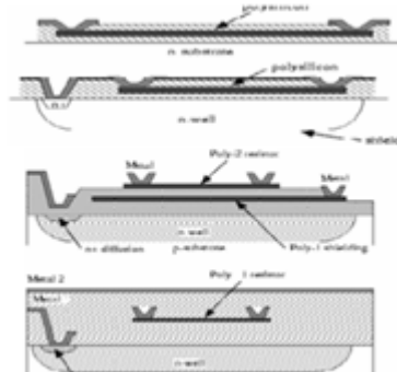
Poly rezistory
